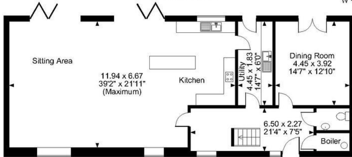
Ground Floor
